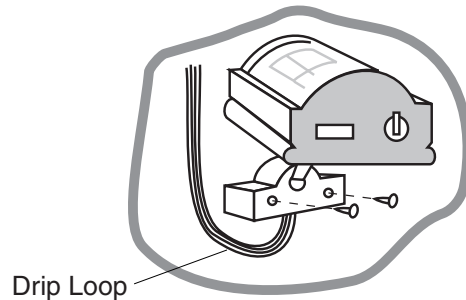
Mounting Sensor
